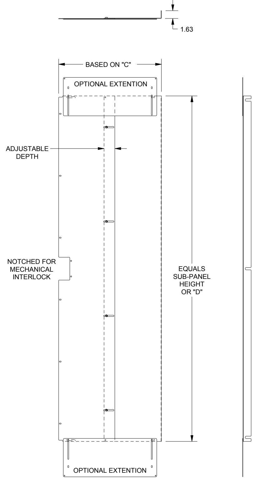
BARRIER DETAIL
