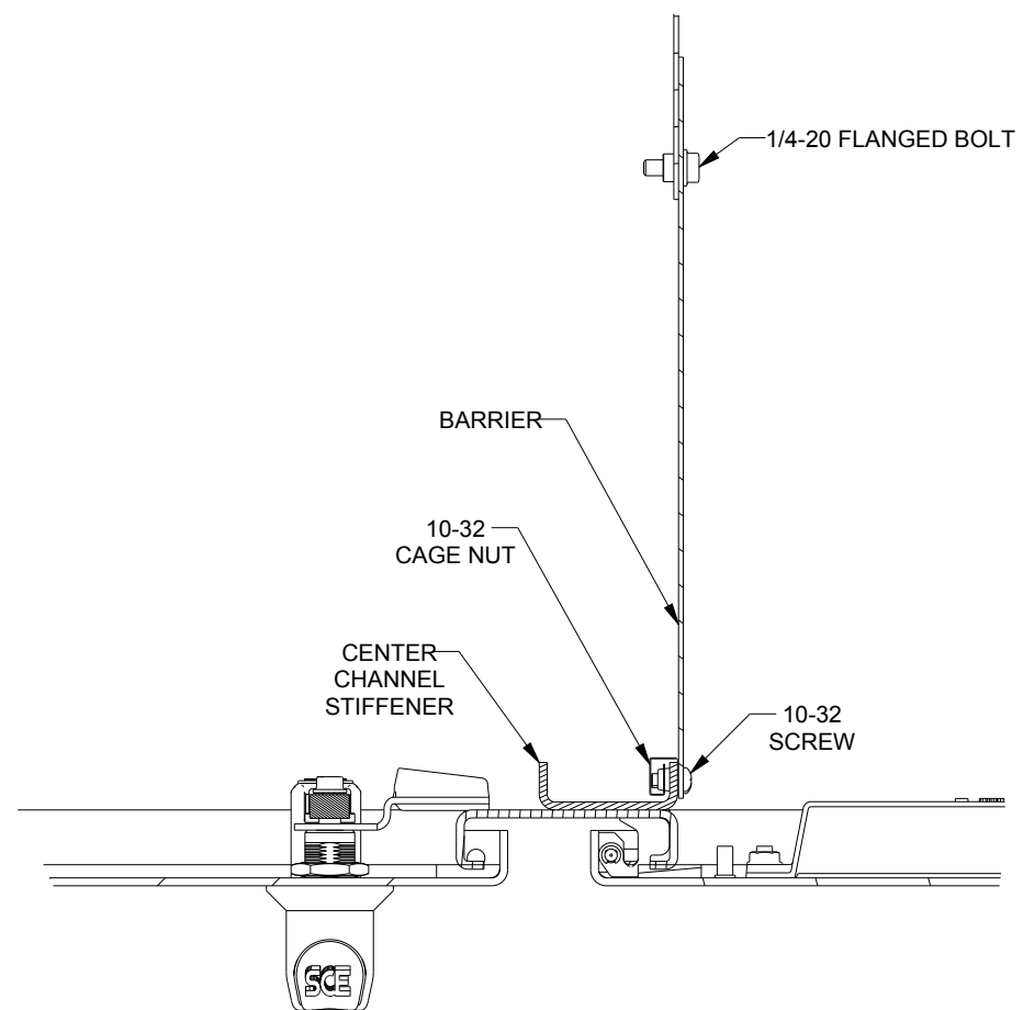
DETAIL A
